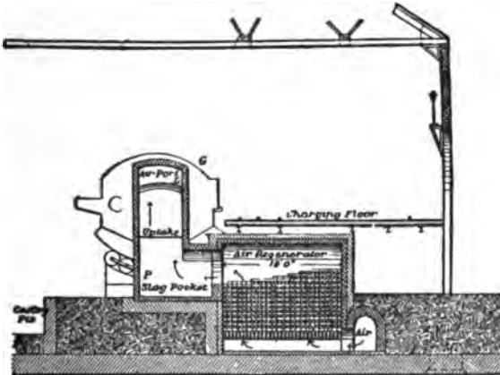
Fig. 101. Section on AB through Up-take, Slag-pocket and Regenerator.
